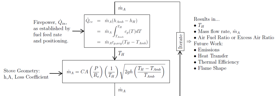
Figure 3: Overall system of equations w/ inputs and outputs.
