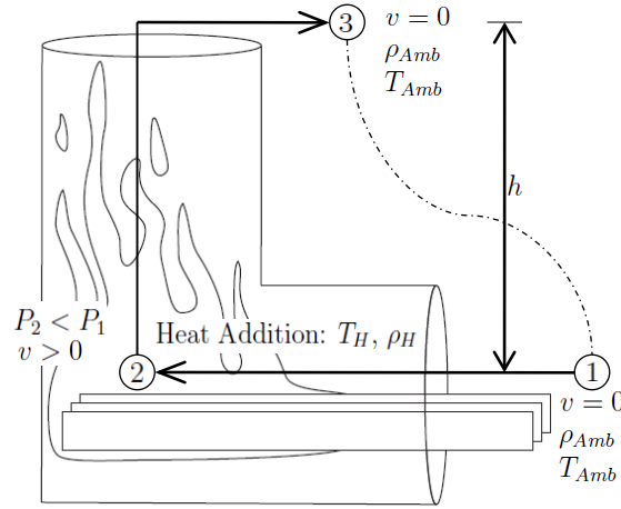
Figure 2: Simplified model setup.
