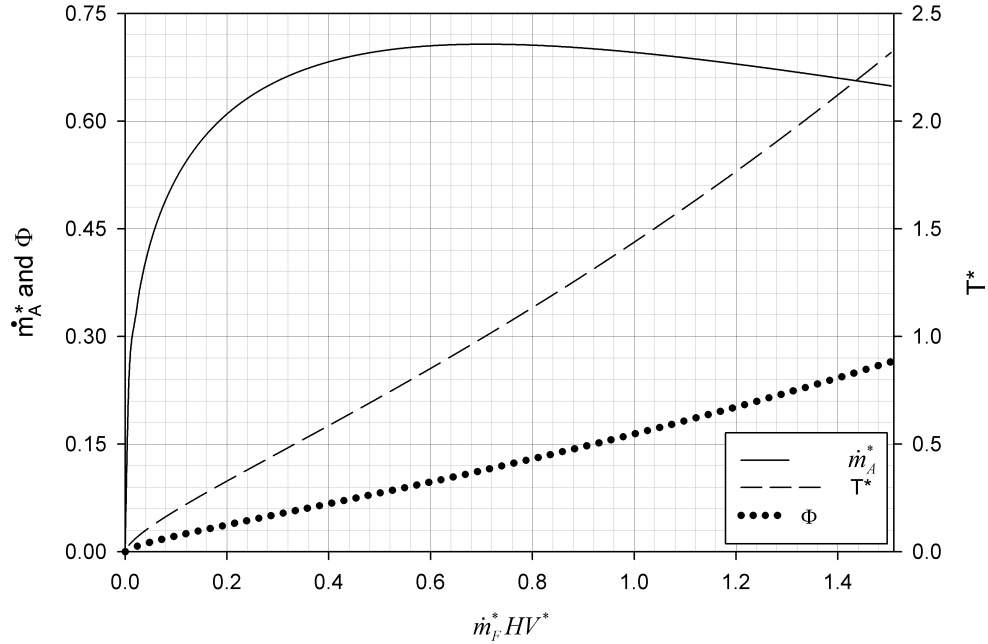
Figure 25: Non-dimensional stove behavior/lookup plot
