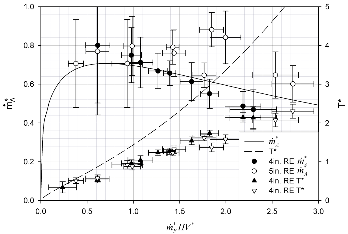
Figure 26: Non-dimensional stove behavior with comparison to validation results.
