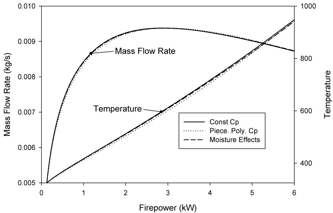
Figure 34: Predicted mass flow rate and temperature behavior for piecewise polynomial specific heat and moisture content effects with comparison to Chapter 3 results.
