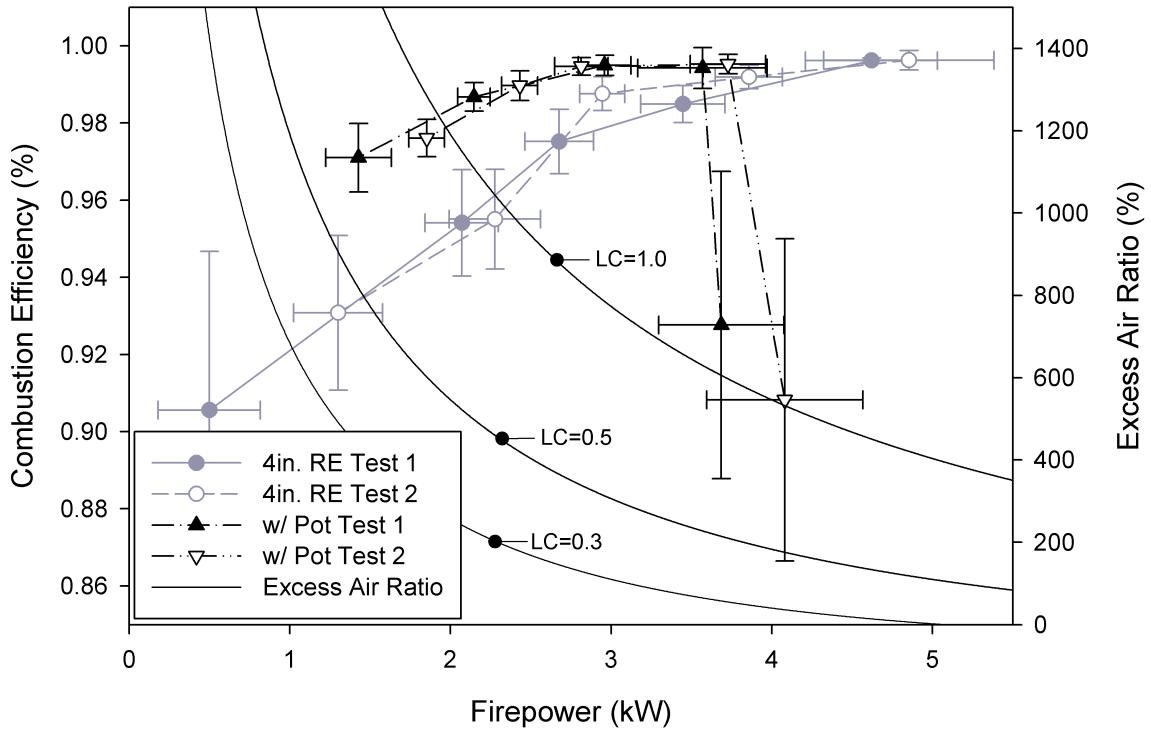
Figure 31: With cook piece CO modified combustion efficiency results with comparison to without cook piece validation results.
