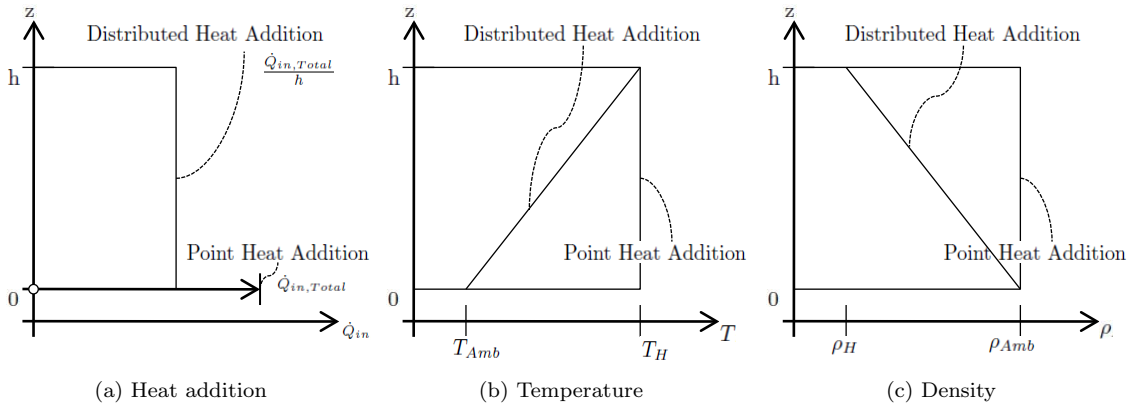
Figure 22: Heat addition, temperature, and density profiles for point and distributed heat addition.
