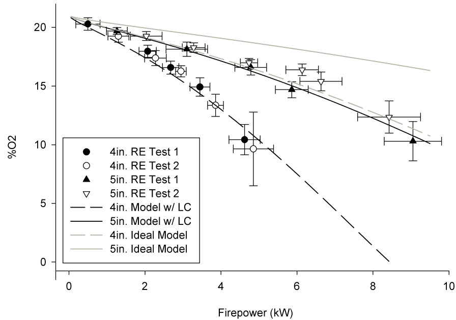
Figure 8: Temporally averaged \%O_2 experimental validation results with comparison to model predicted behavior.
