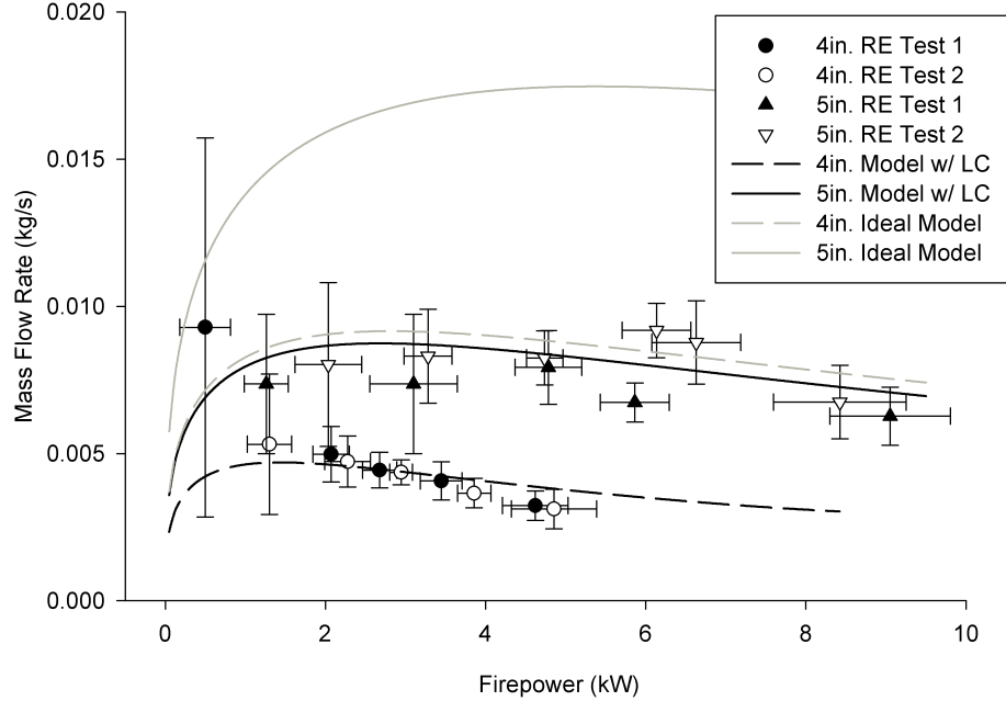
Figure 9: Temporally averaged mass flow rate experimental validation results with comparison to model predicted behavior.
