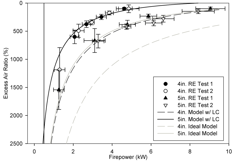
Figure 14: Temporally averaged excess air ratio validation results with comparison to model predicted behavior.
