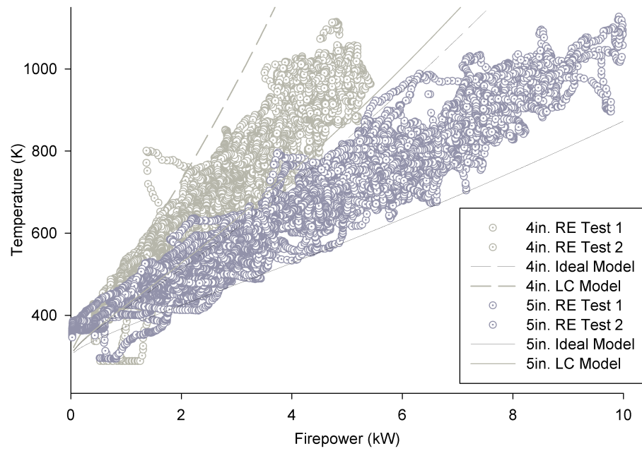
Figure 12: Instantaneous/un-averaged temperature validation results with comparison to model predicted behavior.
