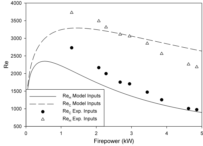
Figure 18: Reynolds number for a 4in. rocket elbow from experimental and model predicted temperature and mass flow rate.
