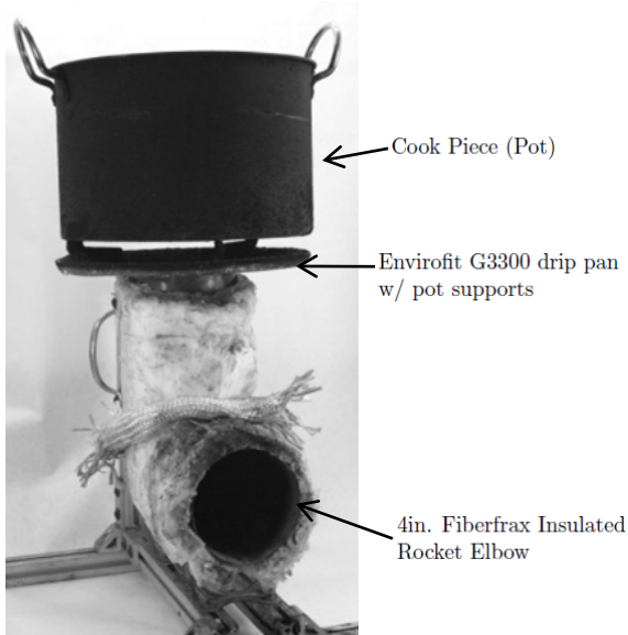
Figure 27: With cook piece validation setup. place.
