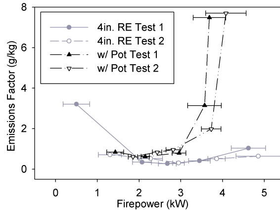
Figure 32: With cook piece PM emissions factor results with comparison to without cook piece results.
