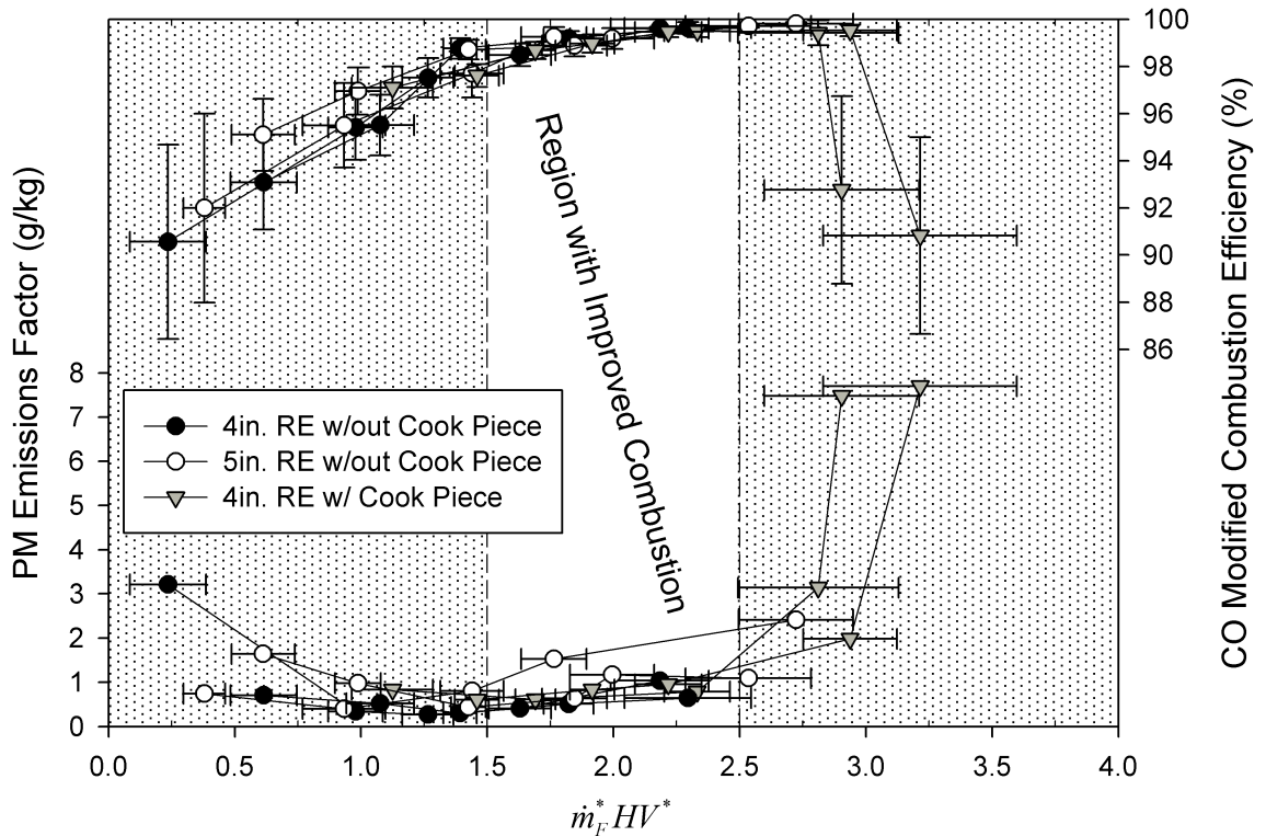
Figure 33: Dimensionless summary of CO MCE and PM EF with improved combustion efficiency region.
