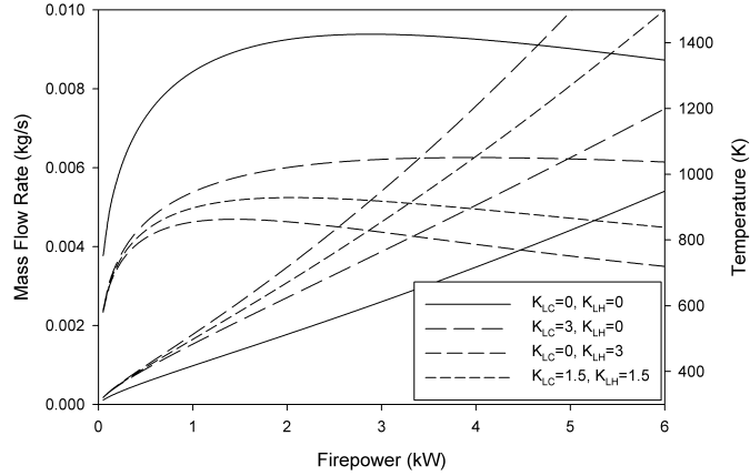
Figure 17: The effect of K_{L,C} and K_{L,H} restriction coefficients
