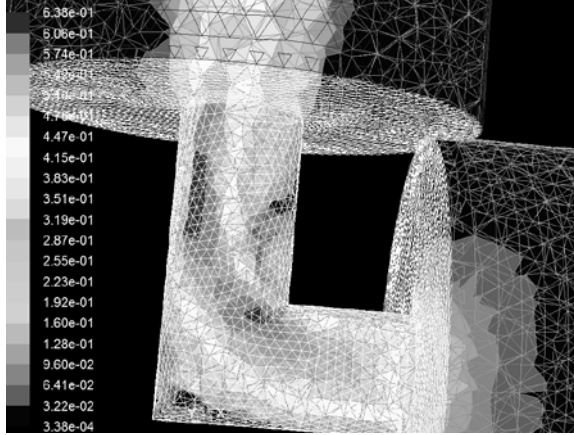
Figure 20: CFD mesh with velocity contour results
