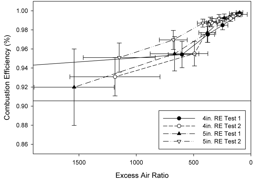
Figure 15: Excess air ratio vs. modified combustion efficiency.
